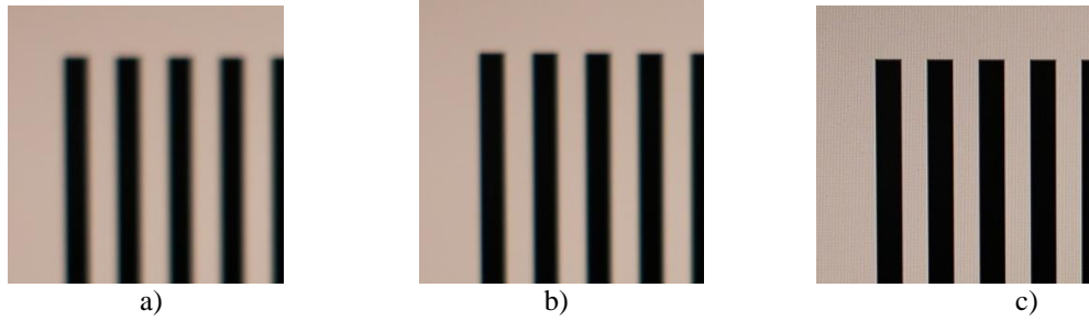
Figure 4. The three captured images with different degrees of blurring. a) Blurred image with \sigma_1 , b) Blurred image with \sigma_2 , c) Focused image.
