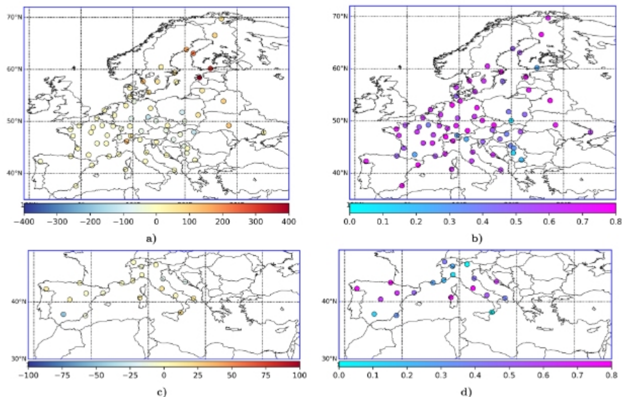
Fig. 14 Bias (left column, panels a,c) and correlation coefficient (right column, panels b,d) of the SILAM birch (upper row, panels a,b) and olive (lower row, panels c, d) forecasts in 2022, as evaluated by Copernicus Atmospheric Monitoring Service 86 . Adopted from CAMS283-2023 report, available for unrestricted use from the CAMS Web portal 86 .
