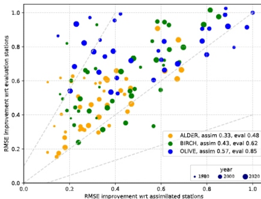
Fig. 8 Summary of L-curve diagnostics for the whole reanalysis. X-axis: RMSE for assimilated stations of the optimal 4D-VAR iteration normalised with that of the 0 th iteration (unconstrained run), y-axis: RMSE for evaluation stations at the optimal iteration normalised with that of the 0 th iteration. On both axes, 1.0 means no improvement due to the data assimilation. Points above the 1:1 line show the years where improvement was higher for assimilated stations than for evaluation ones: large displacement shows an overfit. Two side dashed lines show the slope of 0.5 and 2 with an offset of -0.1 and 0.1 , respectively. The size of the dots is the smallest for 1980 and gradually grows towards 2022. Legend also shows mean RMSE improvement (a fraction of RMSE left after DA).
